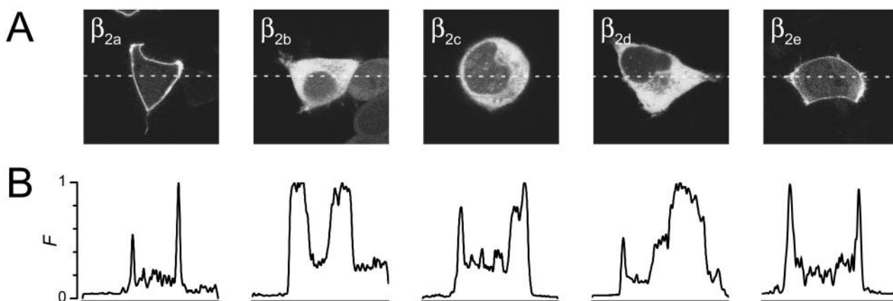
FIGURE 2 Recombinant human \beta_2 splice variants target differentially in HEK 293 cells. (A) Confocal, and (B) line-scan images of \beta_2 -GFP fusion proteins. \beta_{2a} and \beta_{2e} splice variants were localized to the plasma membrane; membrane targeting of \beta_{2a} is caused by palmitoylation of two cysteines in D1. In contrast, \beta_{2b} – \beta_{2d} variants were distributed throughout the cytosol but excluded from the nucleus. F is the normalized fluorescence intensity through the midpoint of images in A.
